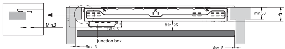
Standard Installation
